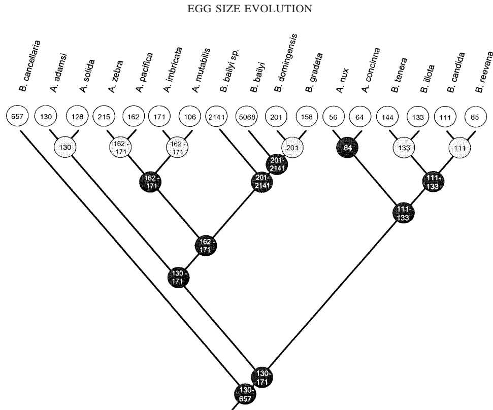
FIG. 4. Phylogeny of 17 arcid bivalve species, showing measured egg sizes of Recent species and egg sizes at ancestral nodes calculated with the linear parsimony algorithm using Mesquite 1.01 (Maddison and Maddison 2004). Tree topology taken from Marko and Moran (2002) with three additional species added using more recent molecular data (described in text). Numbers in white circles at branch tips indicate the measured egg volumes (expressed in cubic microns \times 10^4 ) of 17 Recent arcid species including all six geminate pairs (data also shown in Table 2). Black circles indicate the estimated egg size at ancestral nodes; gray circles are the estimated egg sizes of the immediate ancestors of each geminate pair.
